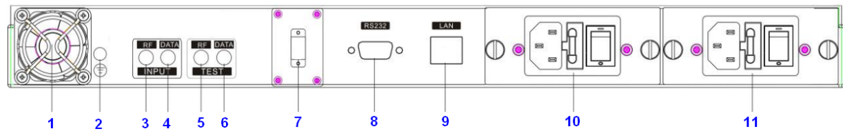
Rear panel
